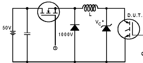
Fig. 13a - Clamped Inductive Load Test Circuit
